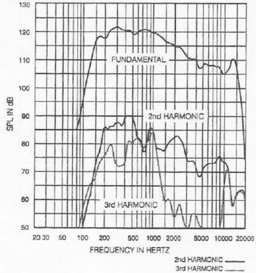
FIGURE 6 — Harmonic Distortion
