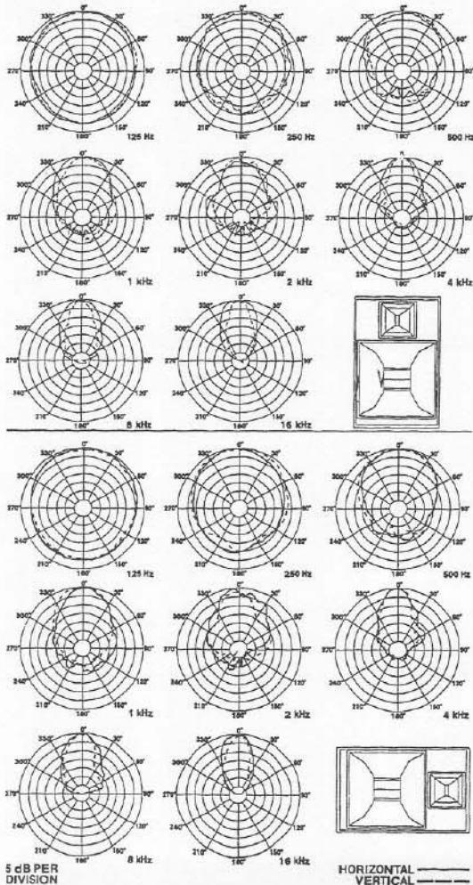
FIGURE 3 — Polar Response
