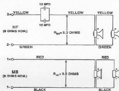
FIGURE 7 — Wiring Diagram
